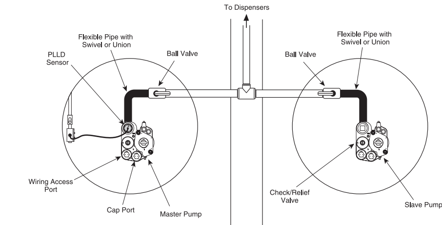
Manifolded systems provide higher flow rates and improved uptime.
